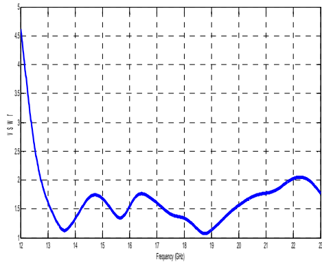
Fig. 5 : VSWR plot of the proposed MIMO
