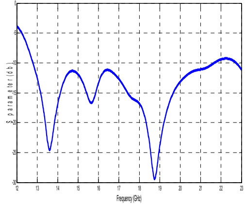
Fig. 2. S_{11} parameters of the proposed antenna.
