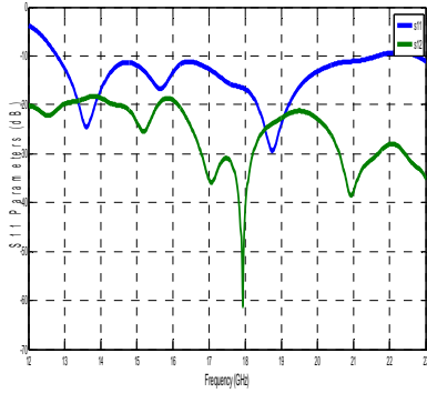
Fig. 4: S_{11} parameters of proposed MIMO System
