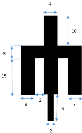
Fig 1: Proposed Fork shaped patch antenna
