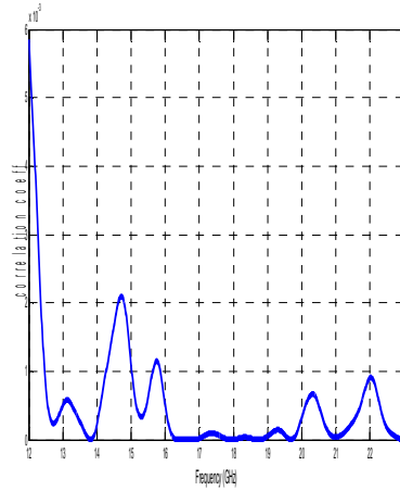
Fig. 6: Correlation Coefficient Plot of the Proposed MIMO
